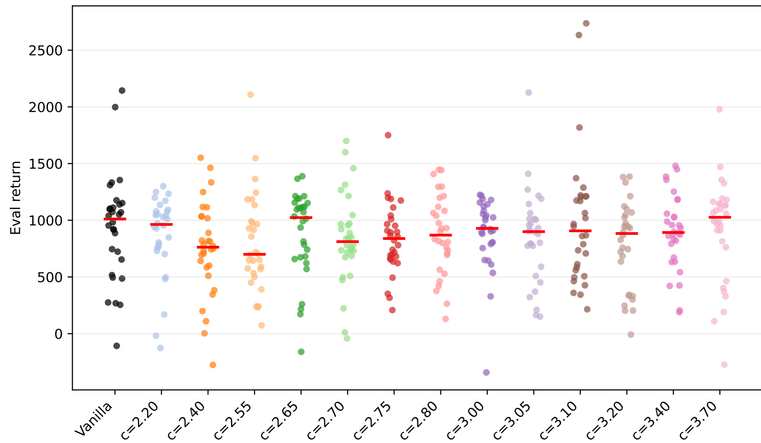
HalfCheetah-v4 mass factor=0.5: seed scatter (raw)
