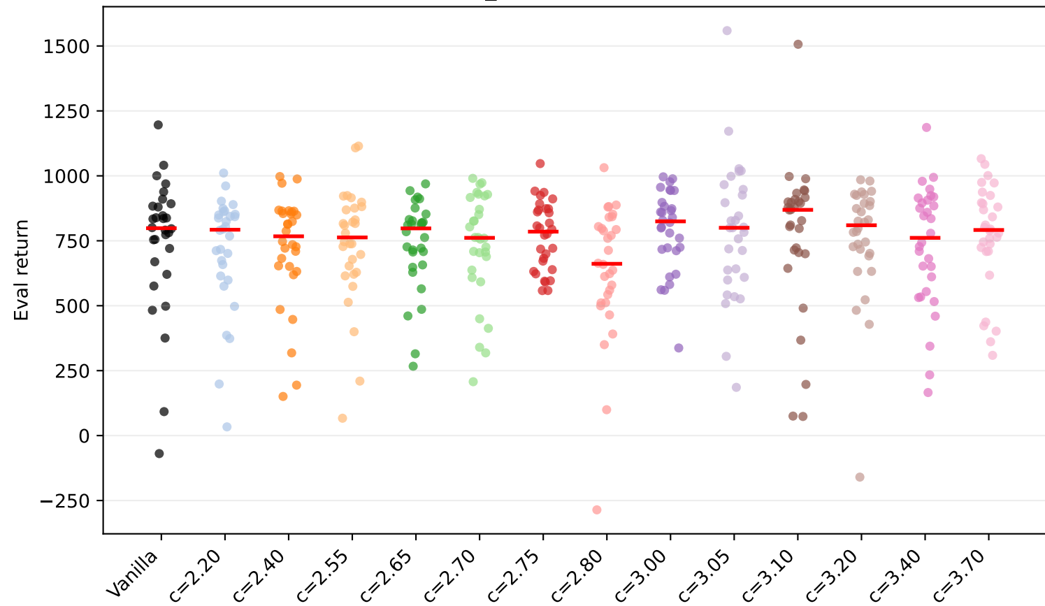
HalfCheetah-v4 state_noise factor=0.5: seed scatter (raw)
