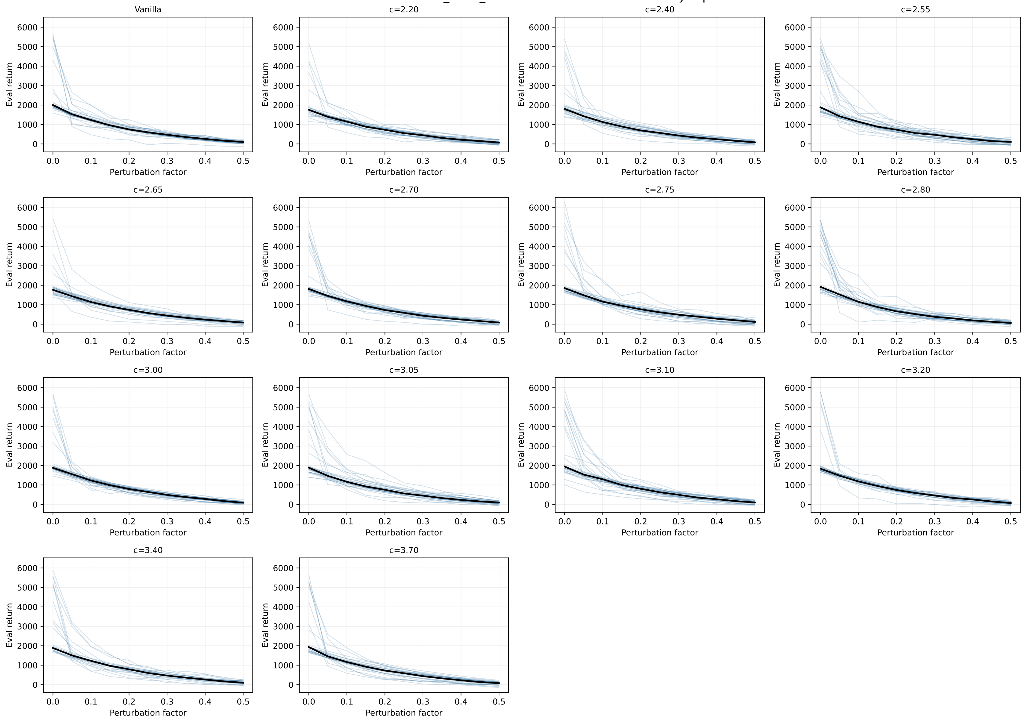
HalfCheetah-v4 action_noise_bernoulli: 30 seed return curves by cap
