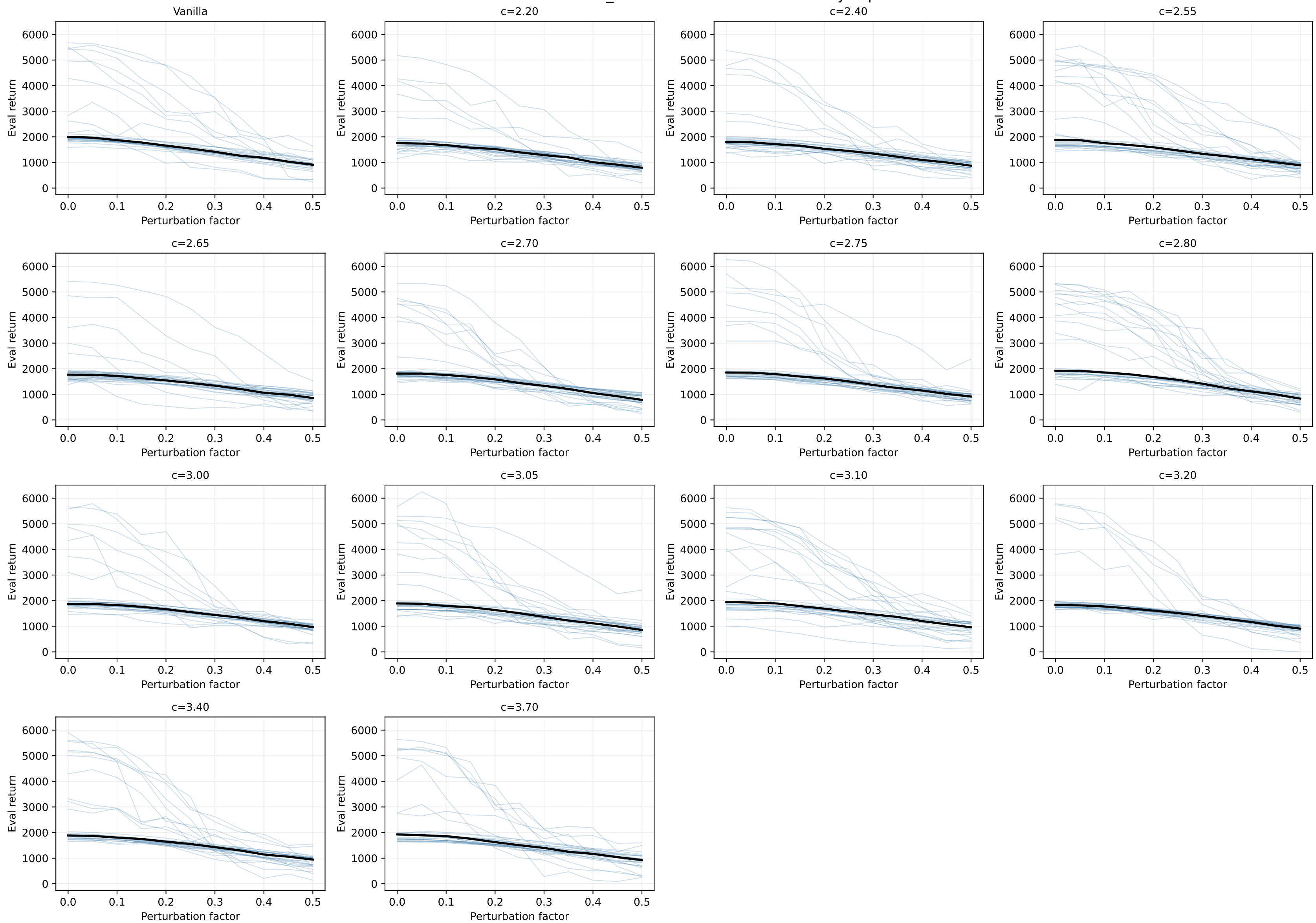
HalfCheetah-v4 action_noise: 30 seed return curves by cap
