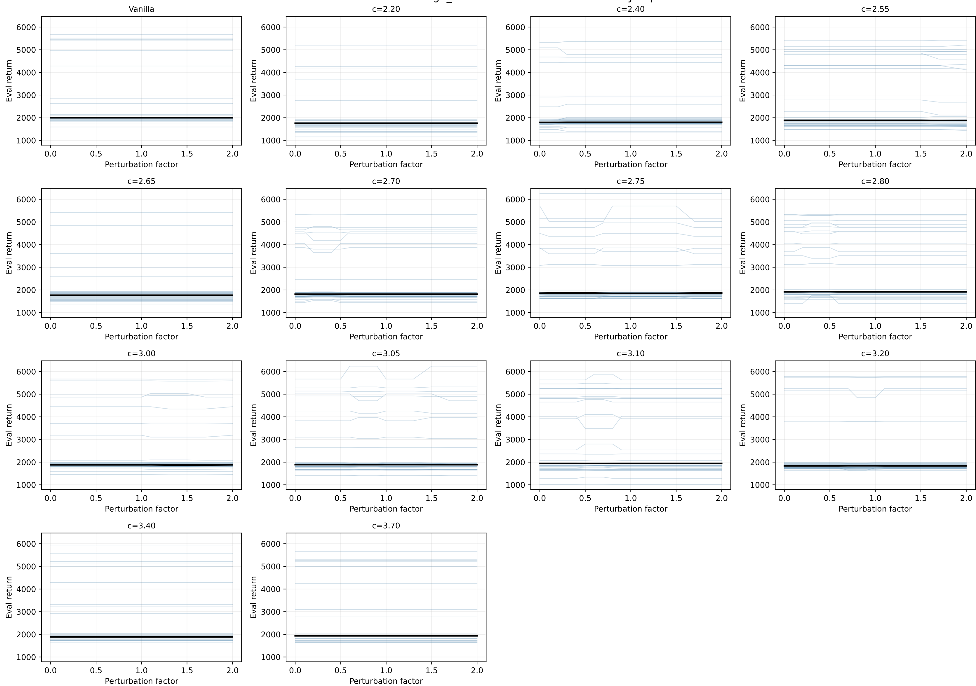
HalfCheetah-v4 bthigh_friction: 30 seed return curves by cap
