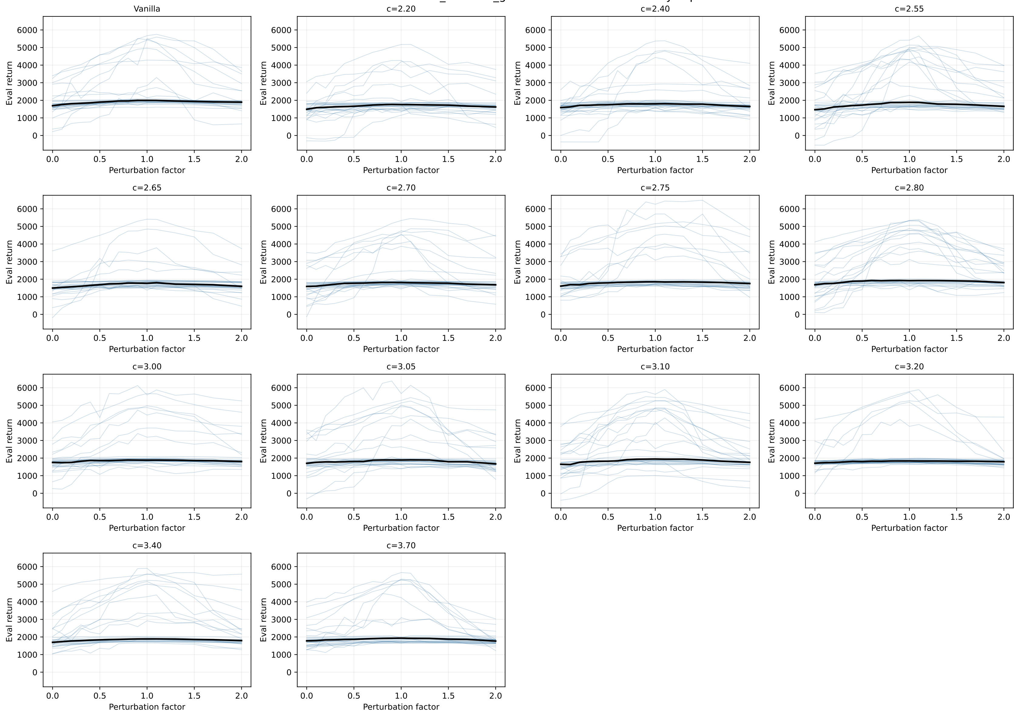
HalfCheetah-v4 ffoot_actuator_gain: 30 seed return curves by cap
