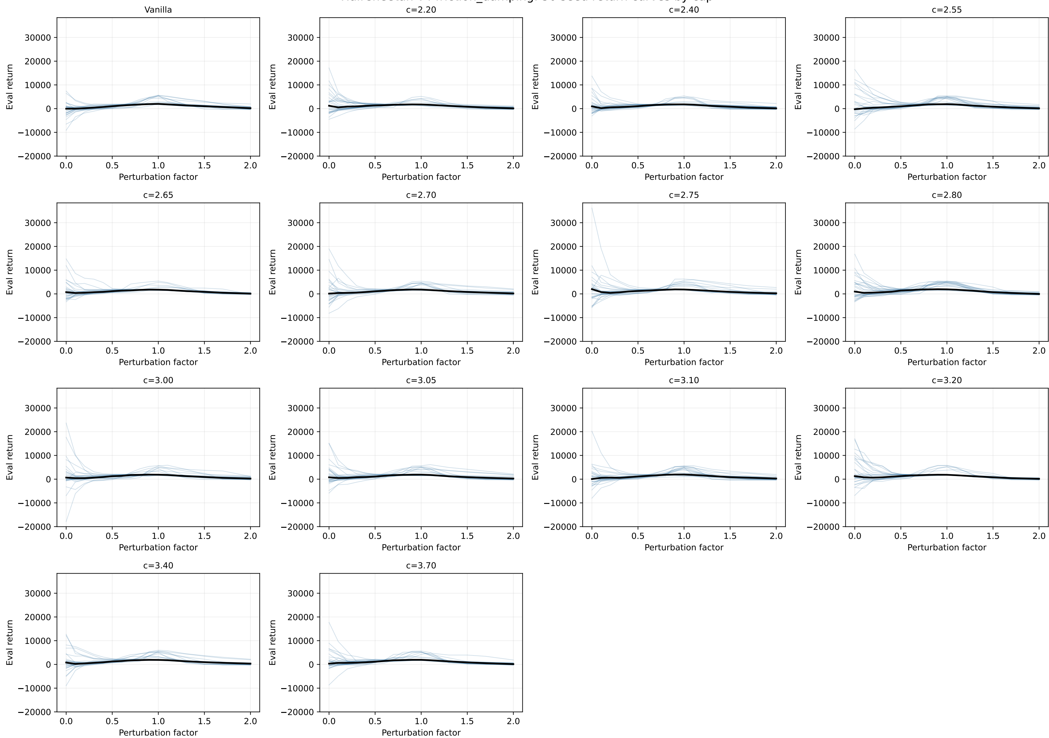
HalfCheetah-v4 friction_damping: 30 seed return curves by cap
