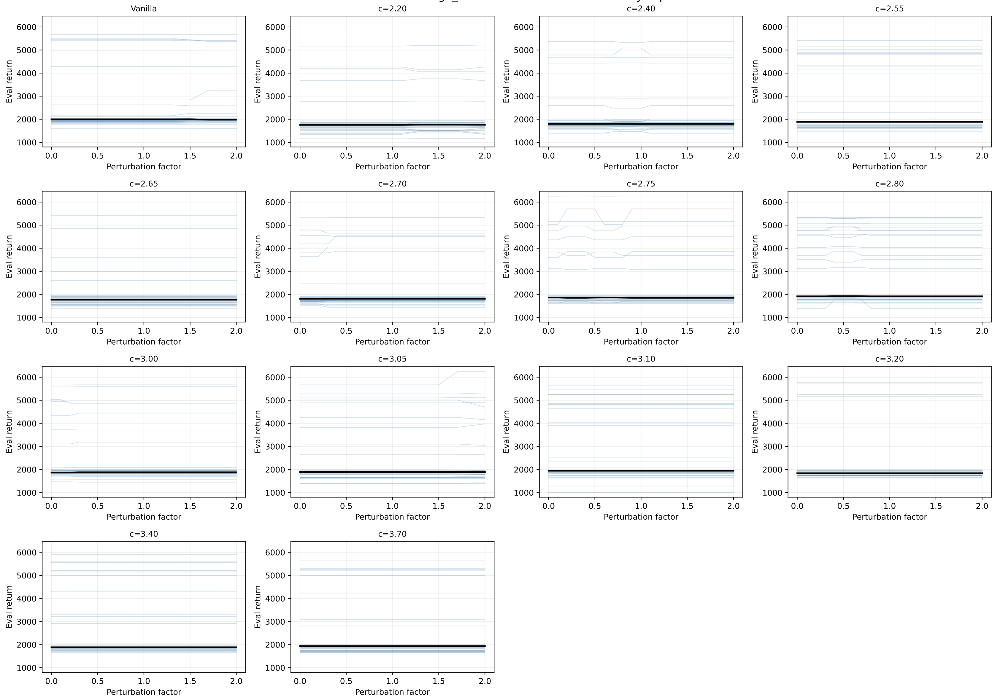
HalfCheetah-v4 fthigh_friction: 30 seed return curves by cap
