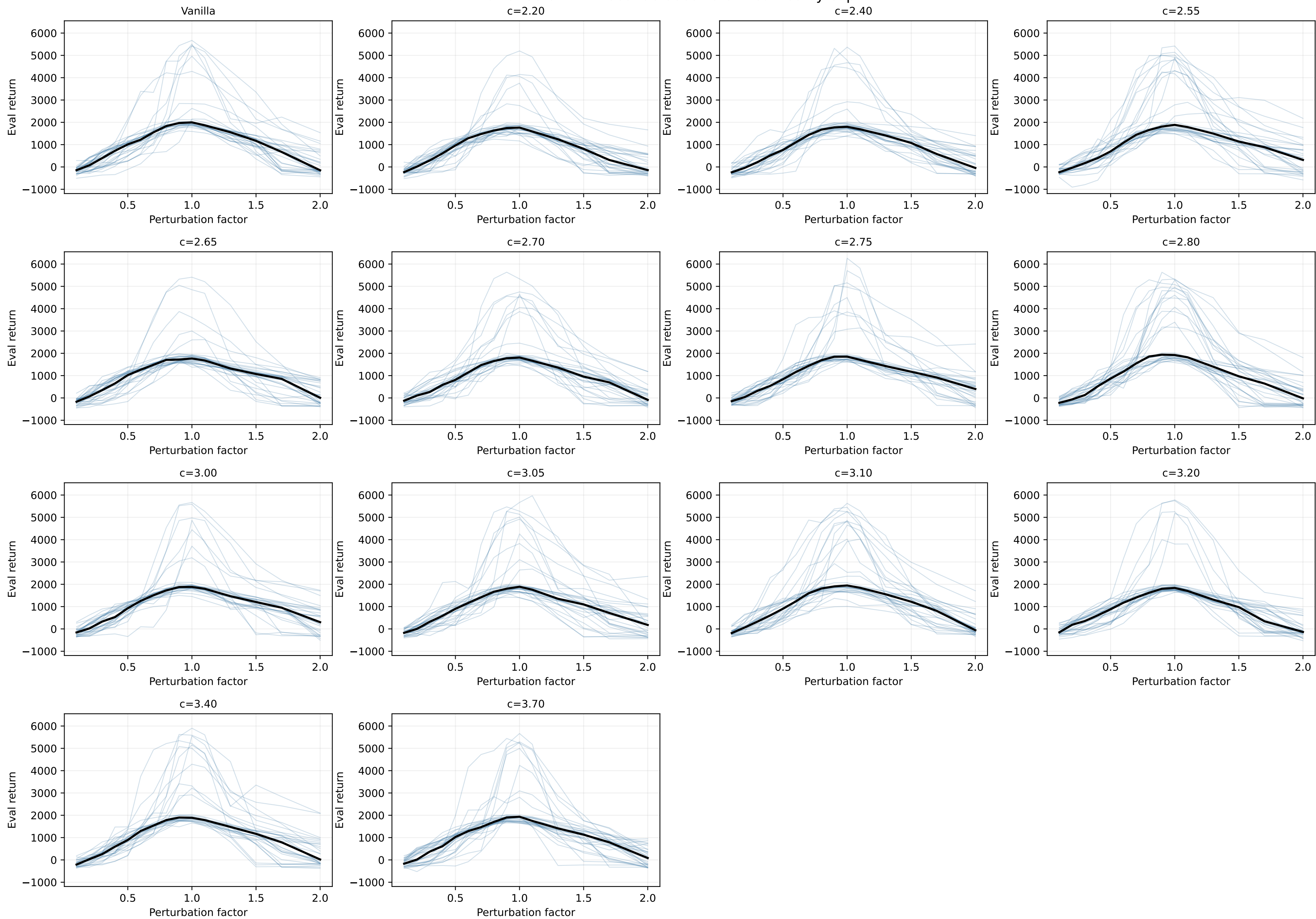
HalfCheetah-v4 mass: 30 seed return curves by cap
