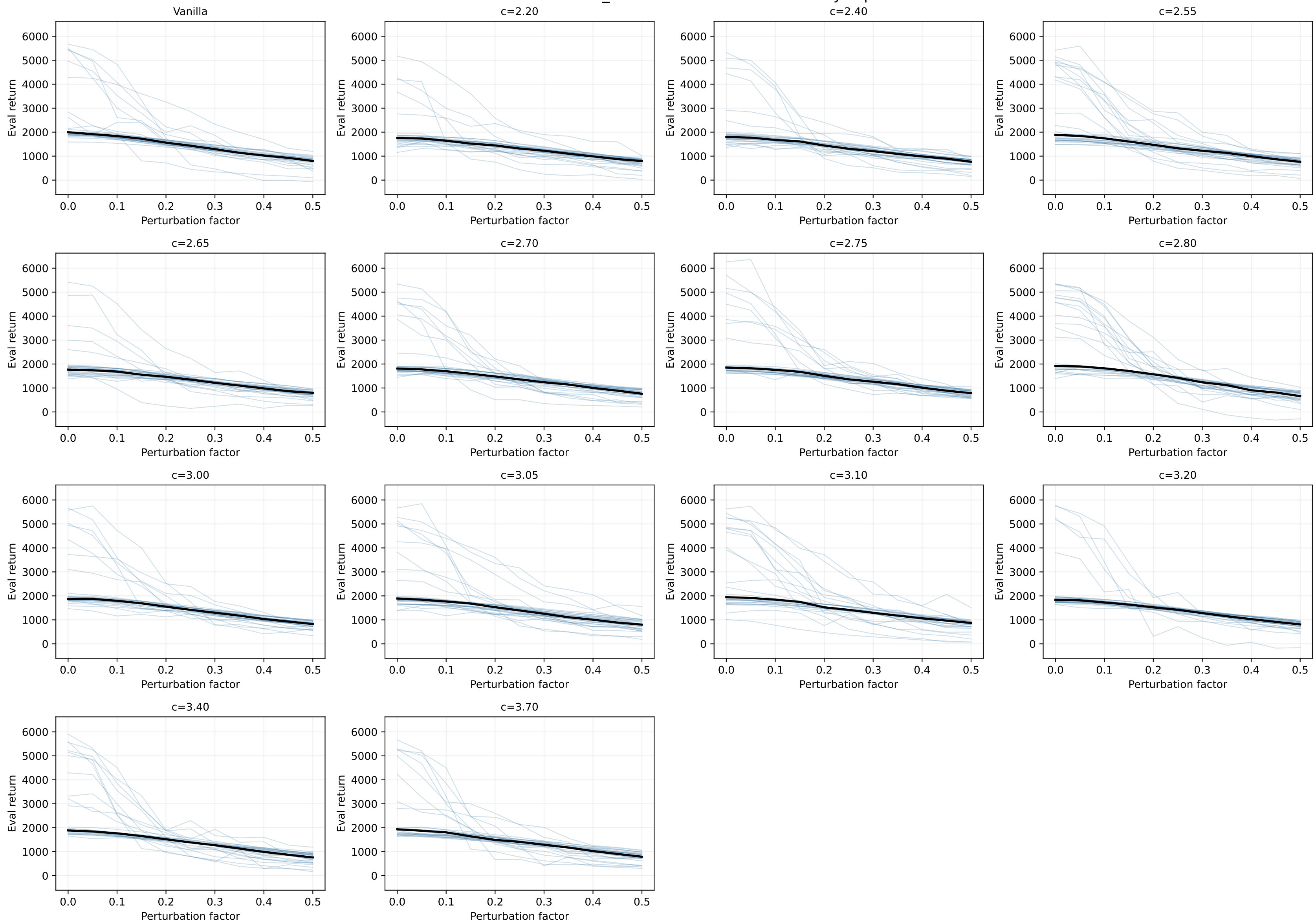
HalfCheetah-v4 state_noise: 30 seed return curves by cap
