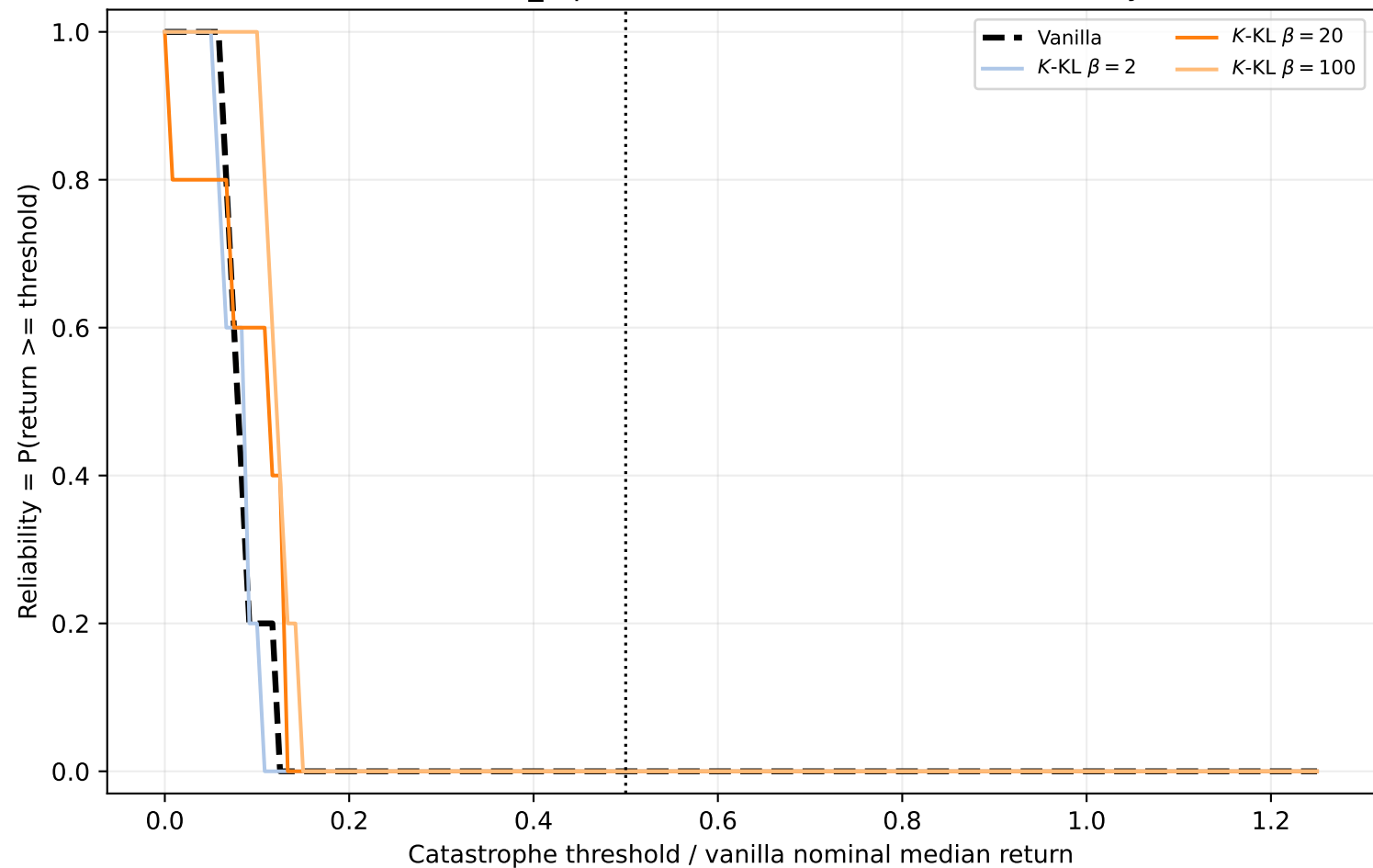
Walker2d-v4 action_replace factor=0.5: robustness reliability curve
