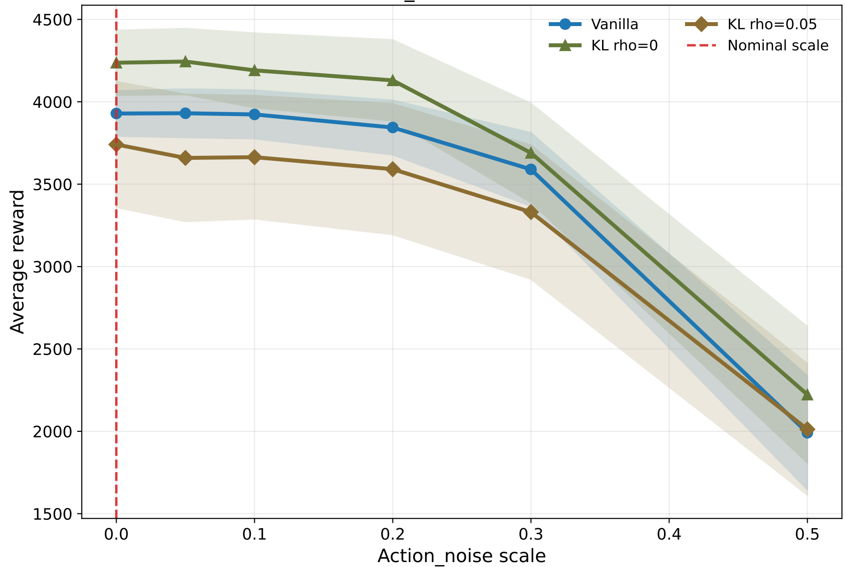
Action_noise robustness
