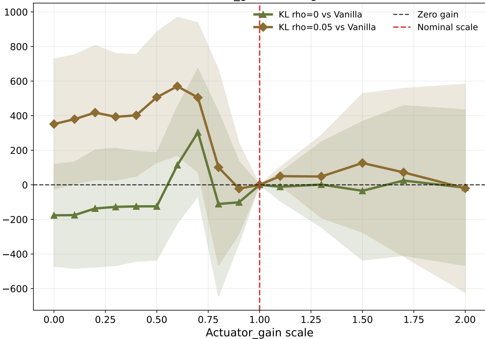
Actuator_gain robust gain
