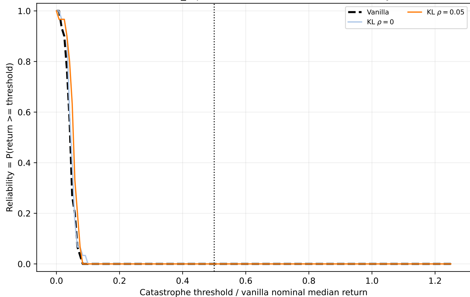
Walker2d-v5 action_replace factor=0.5: robustness reliability curve
