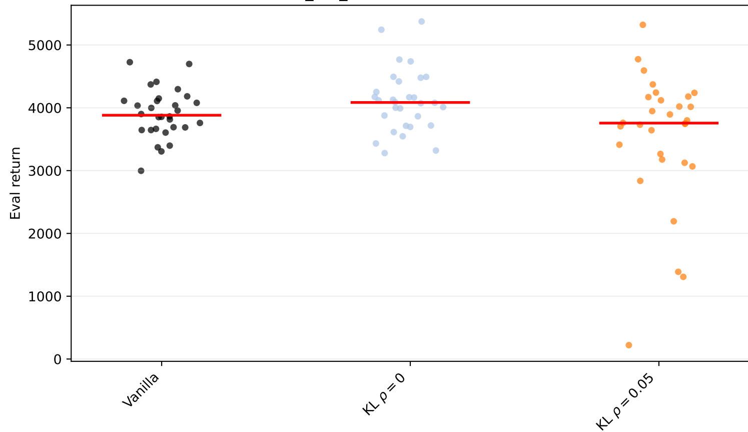
Walker2d-v5 foot_left_friction factor=0.5: seed scatter (raw)
