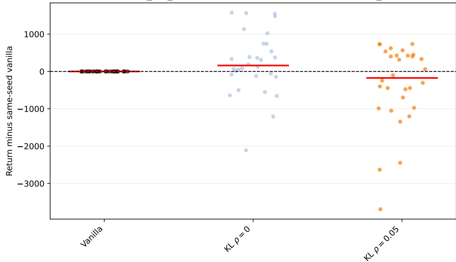
Walker2d-v5 leg_left_damping factor=0.5: seed scatter (vanilla_subtracted)
