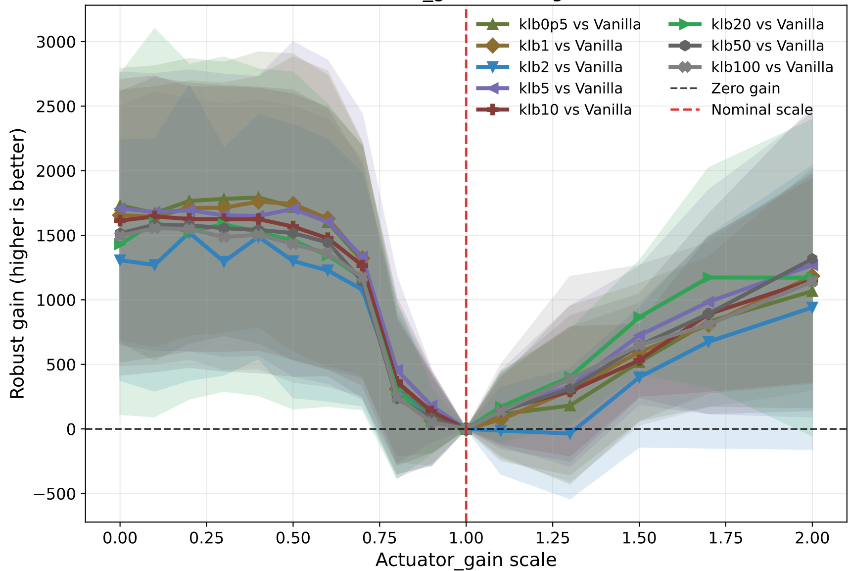
Actuator_gain robust gain
