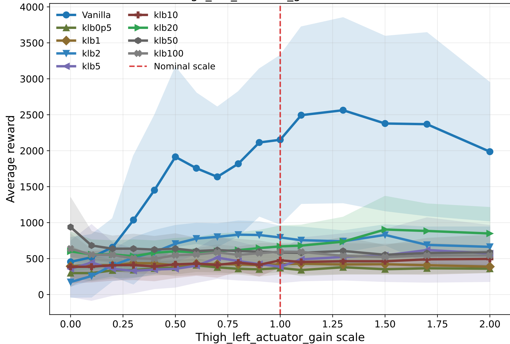
Thigh_left_actuator_gain robustness
