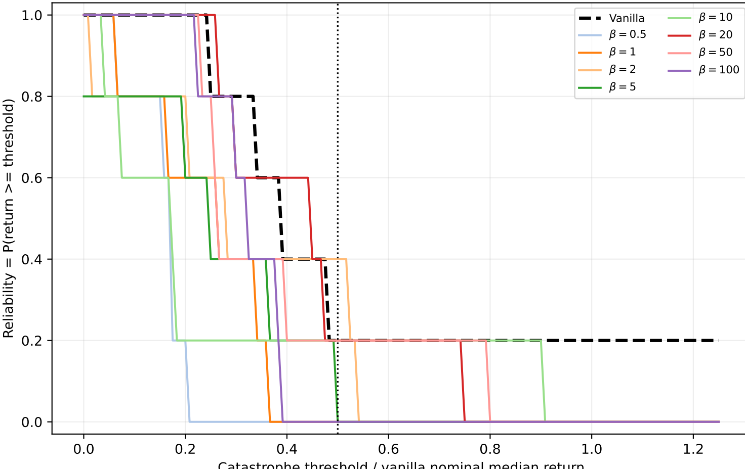
Walker2d-v4 mass damping factor=0.5: robustness reliability curve
