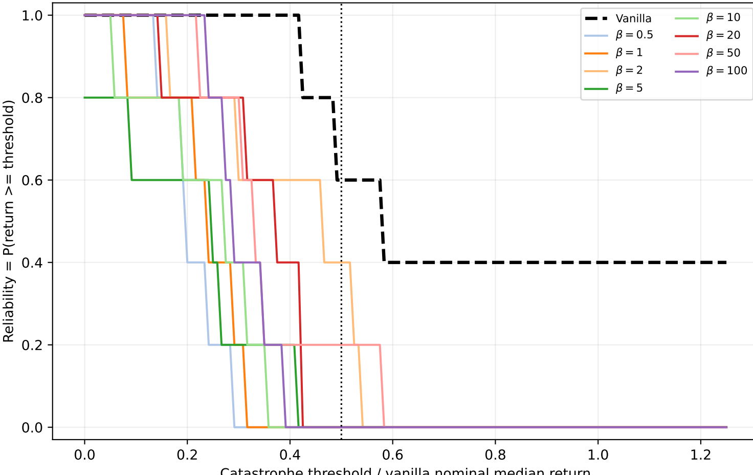
Walker2d-v4 thigh left actuator gain factor=0.5: robustness reliability curve
