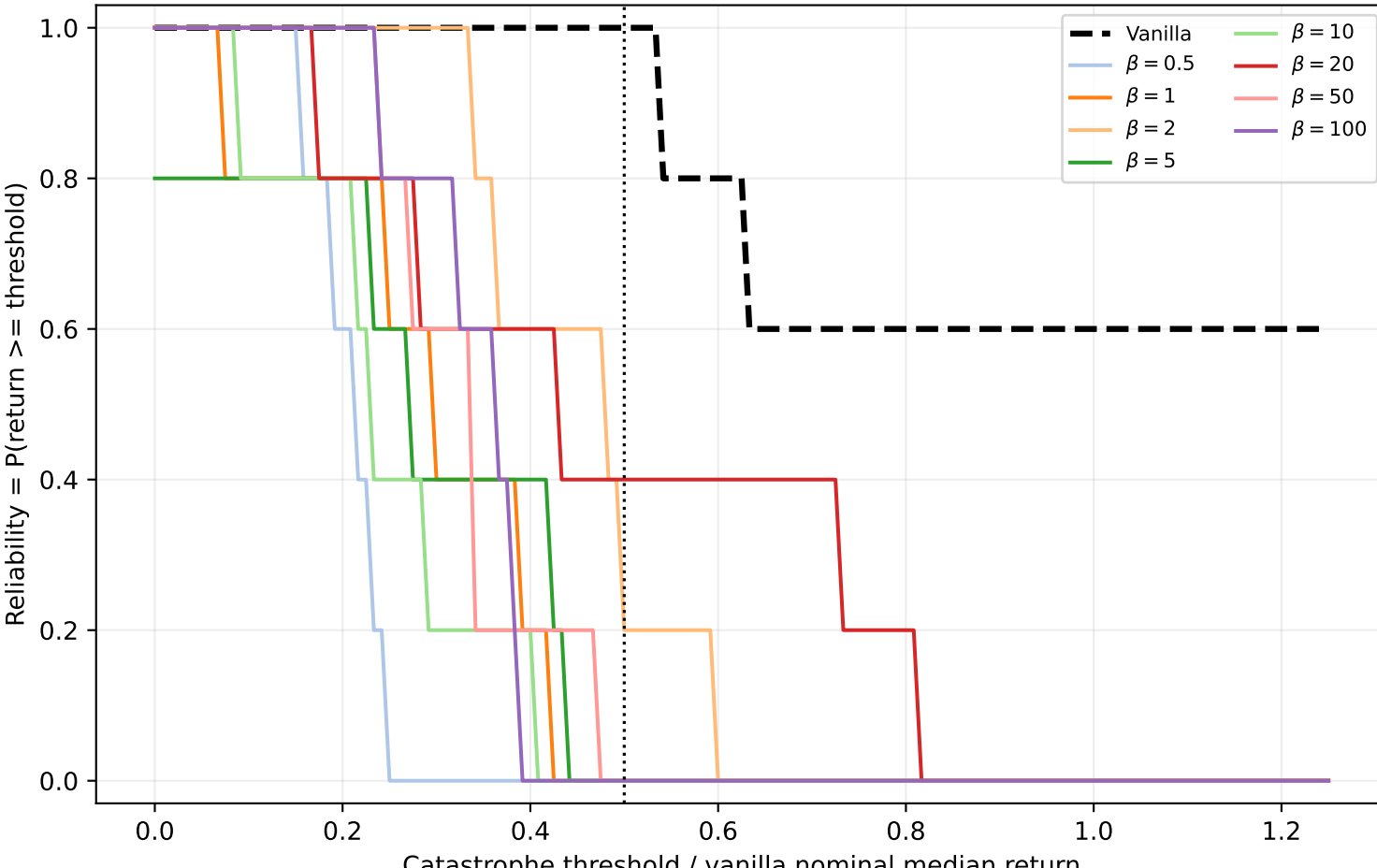
Walker2d-v4 thigh left mass factor=0.5: robustness reliability curve
