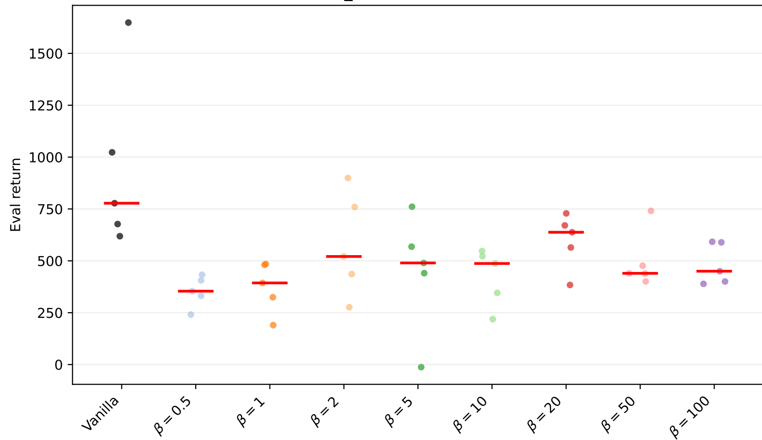
Walker2d-v4 action_noise factor=0.5: seed scatter (raw)
