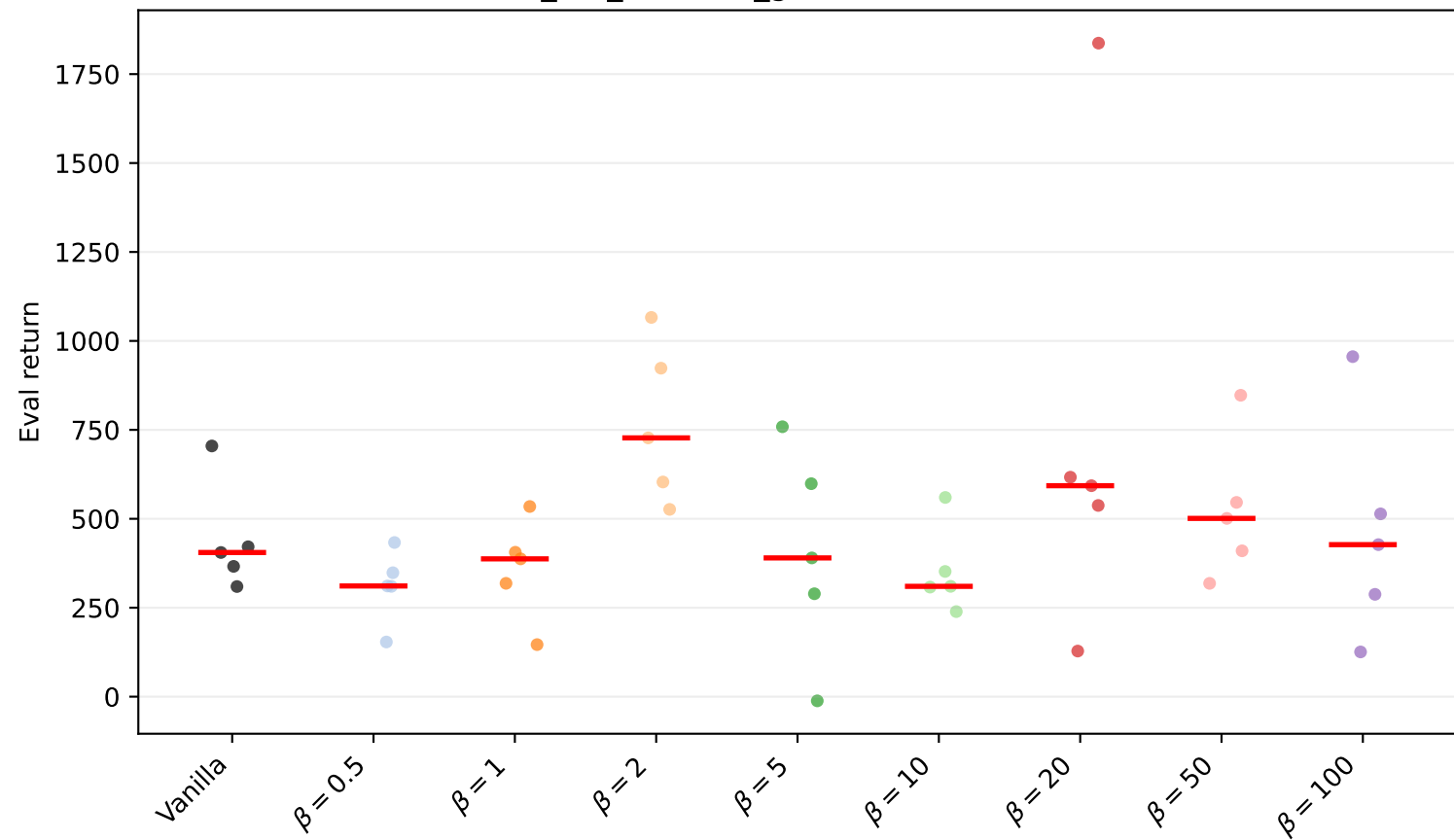
Walker2d-v4 foot_left_actuator_gain factor=0.5: seed scatter (raw)
