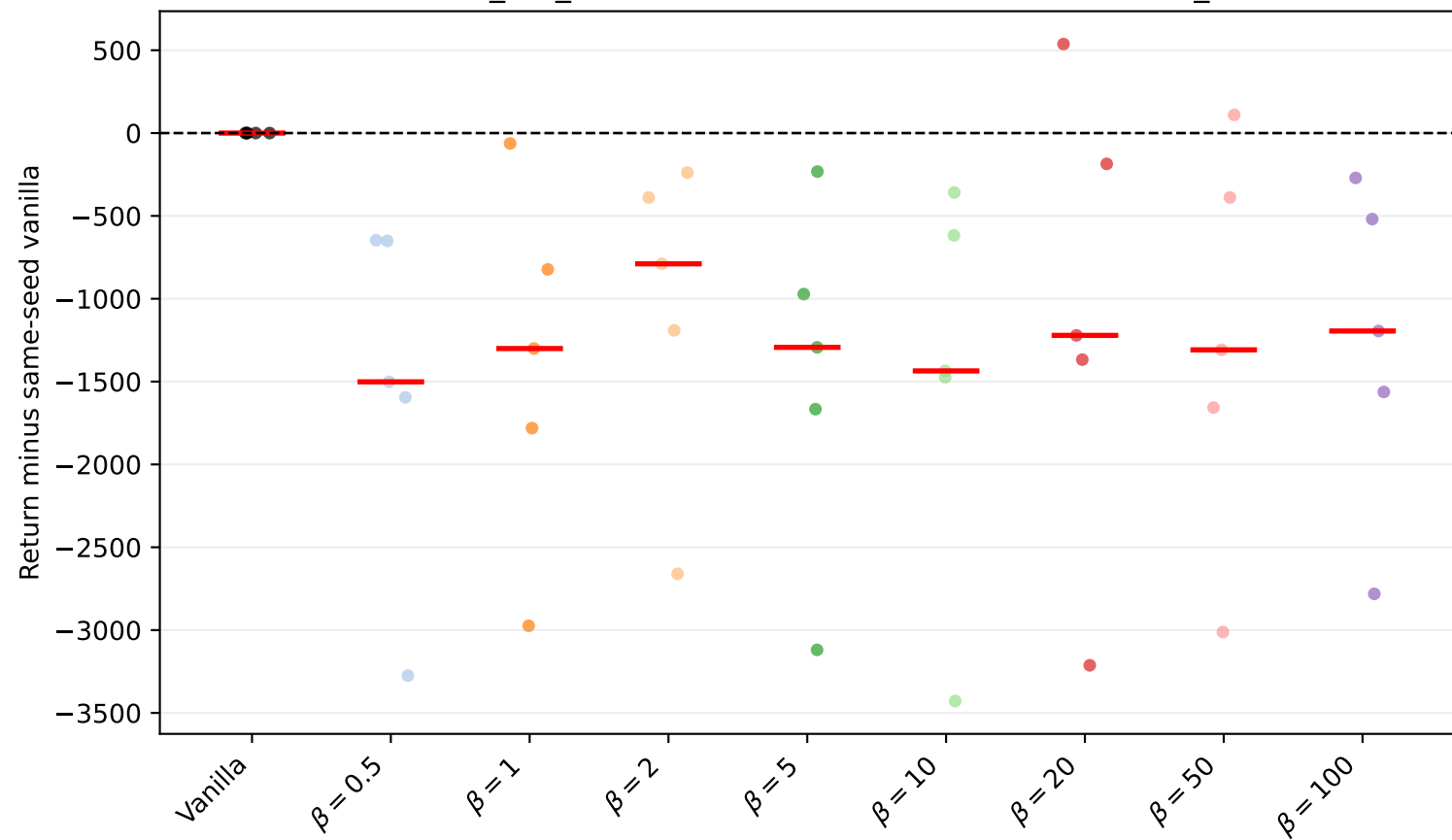
Walker2d-v4 foot_left_friction factor=0.5: seed scatter (vanilla_subtracted)
