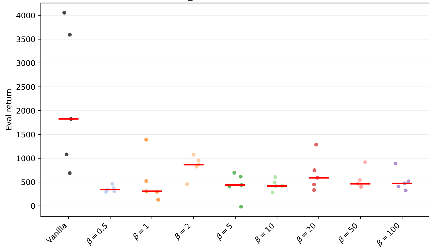
Walker2d-v4 friction_damping factor=0.5: seed scatter (raw)
