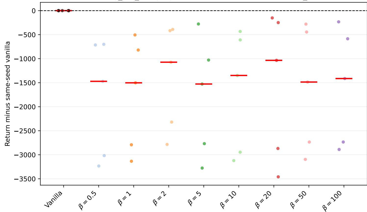
Walker2d-v4 leg_left_damping factor=0.5: seed scatter (vanilla_subtracted)
