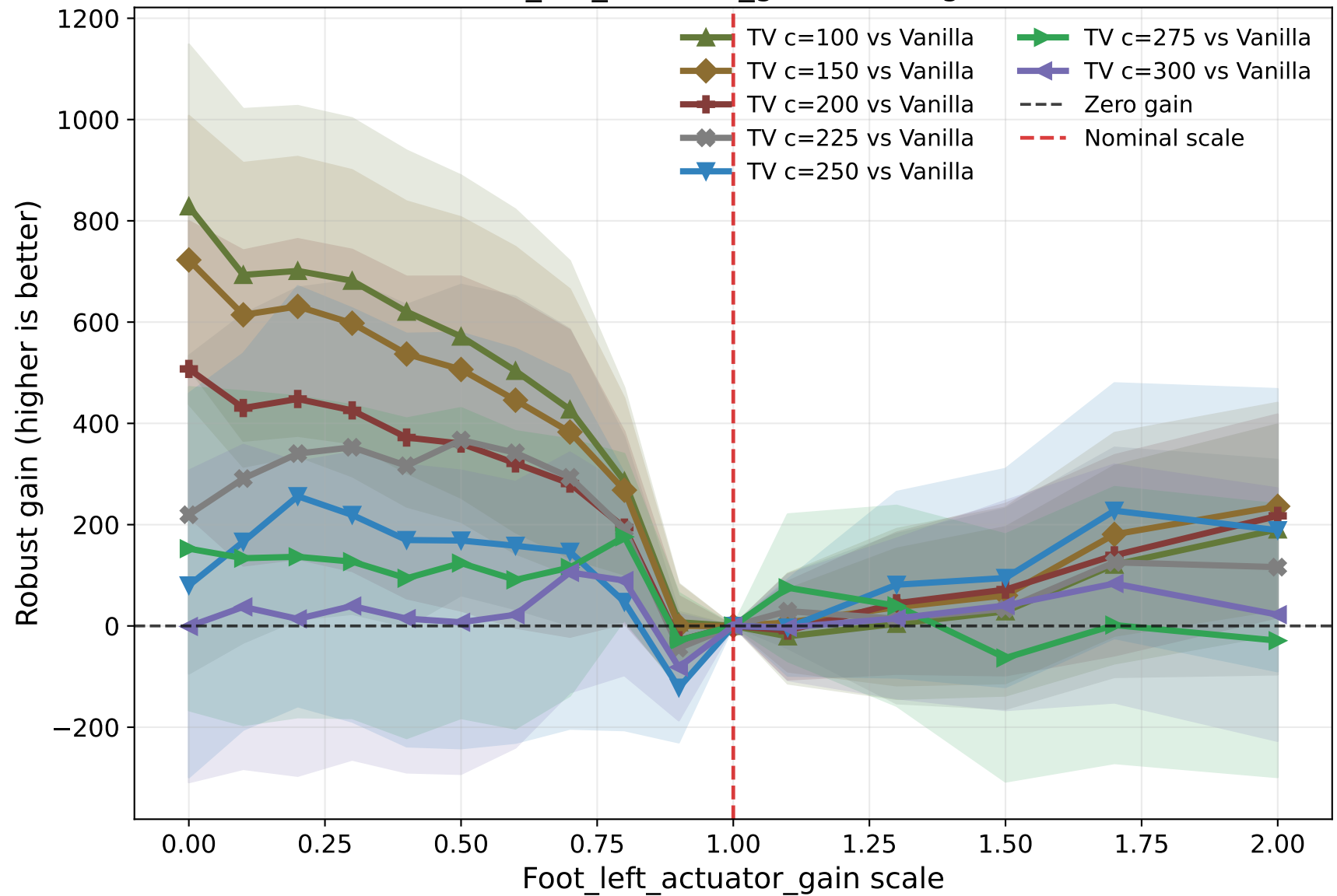
Foot_left_actuator_gain robust gain
