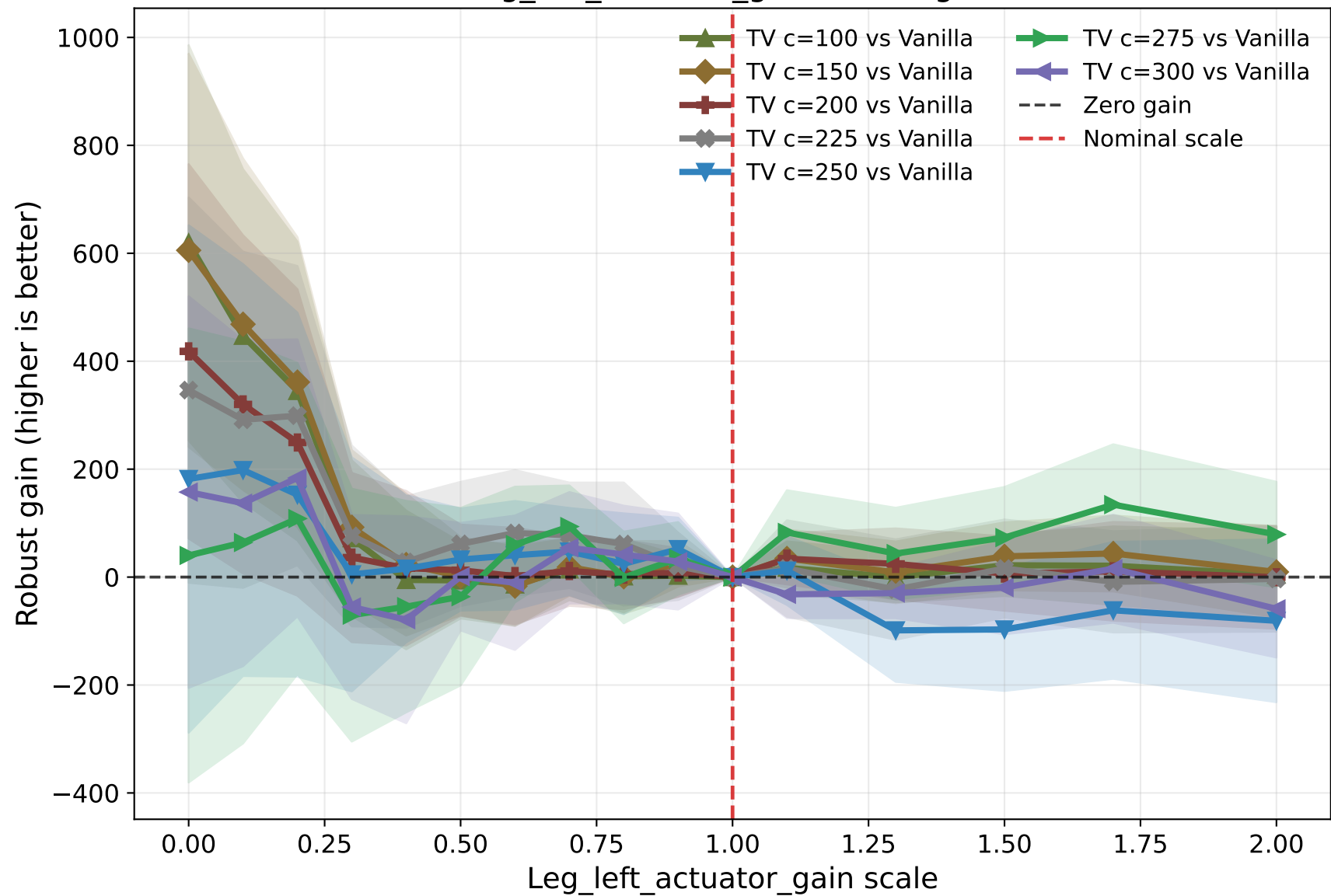
Leg_left_actuator_gain robust gain
