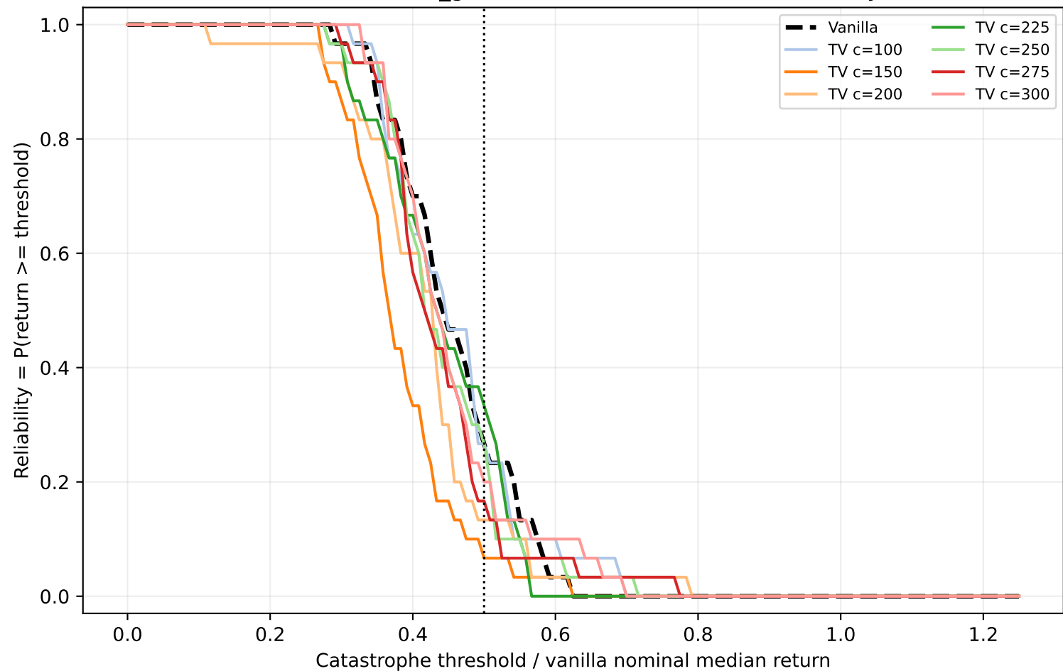
Walker2d-v4 actuator_gain factor=0.5: robustness reliability curve
