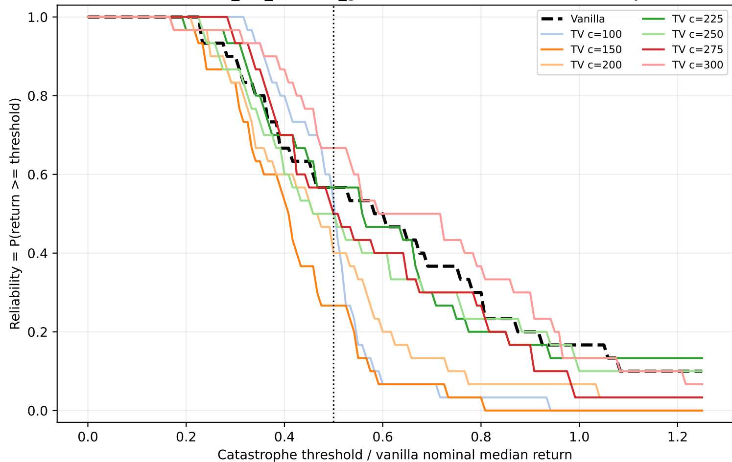
Walker2d-v4 foot_left_actuator_gain factor=0.5: robustness reliability curve
