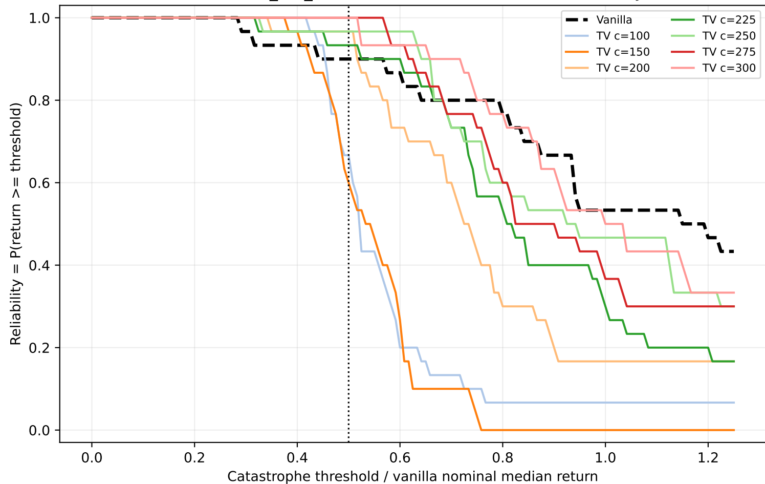
Walker2d-v4 foot_left_friction factor=0.5: robustness reliability curve
