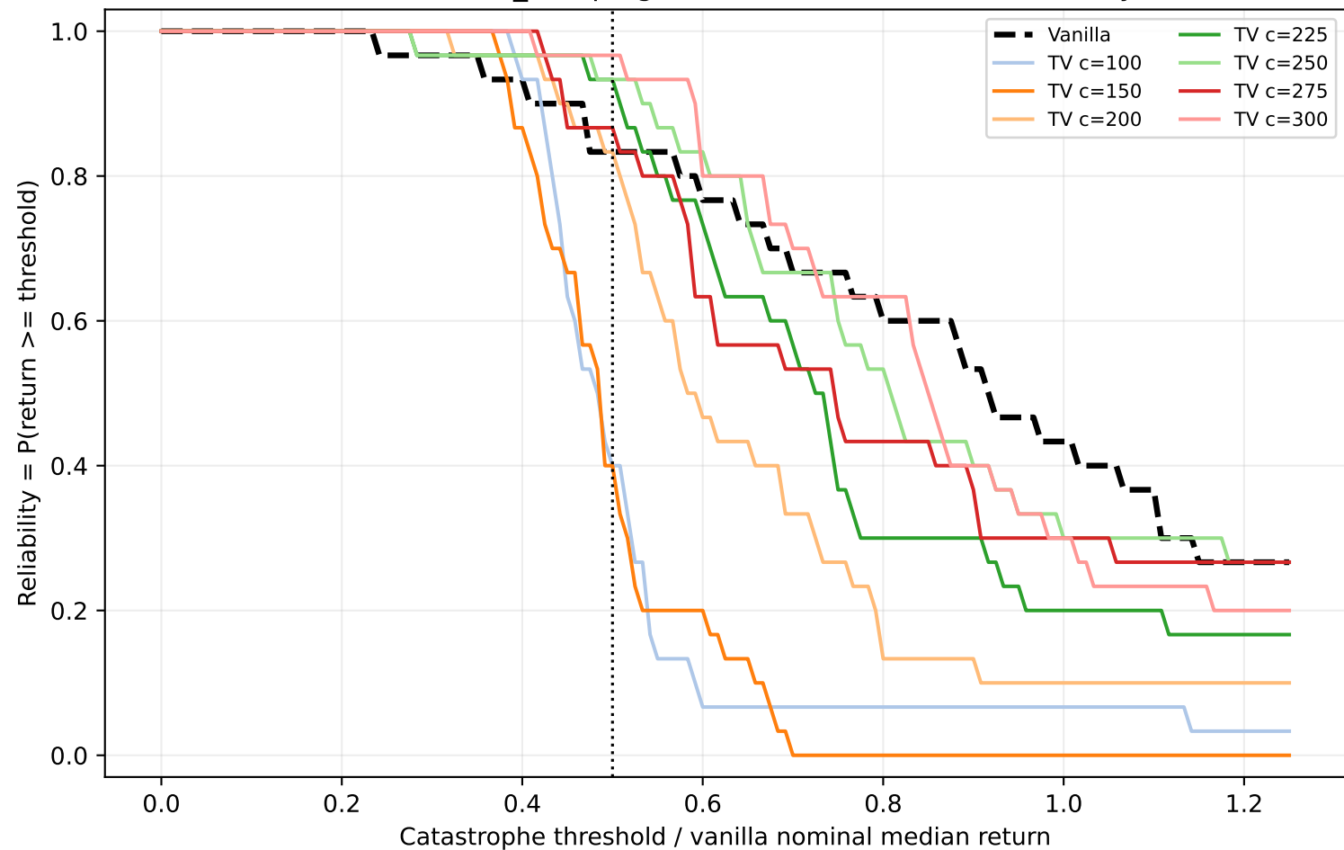
Walker2d-v4 friction_damping factor=0.5: robustness reliability curve
