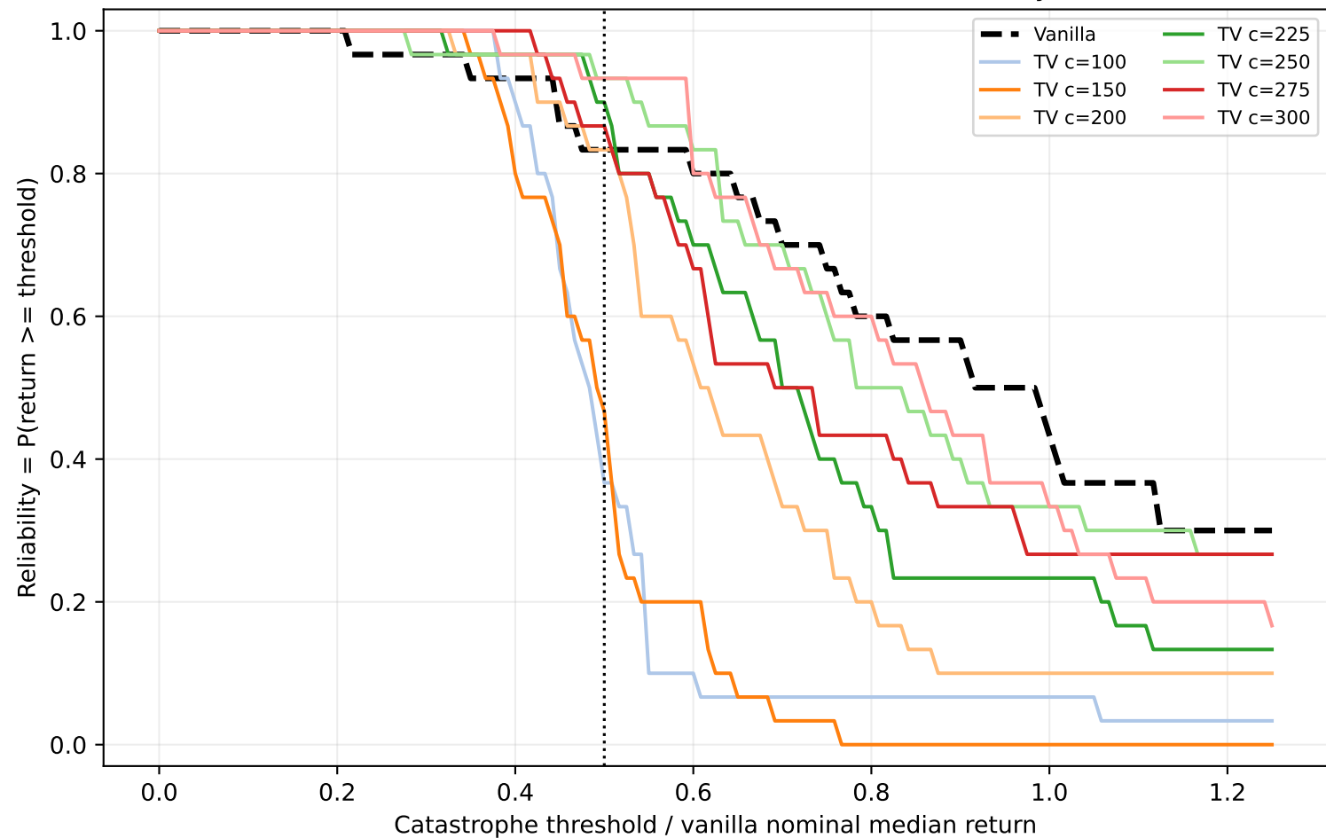
Walker2d-v4 friction factor=0.5: robustness reliability curve
