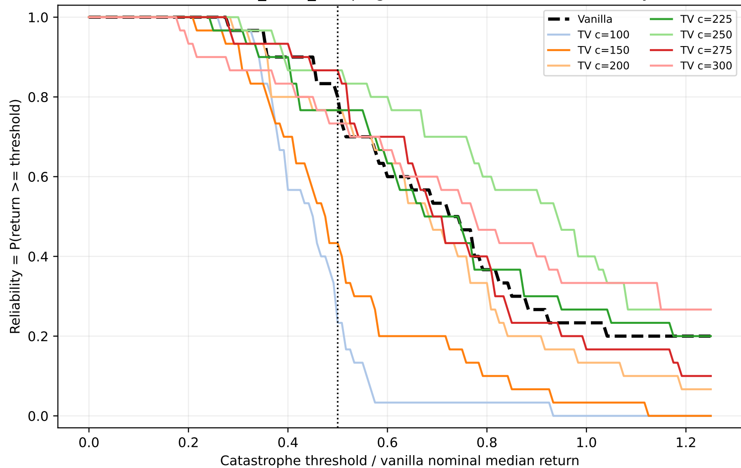
Walker2d-v4 friction_mass_damping factor=0.5: robustness reliability curve
