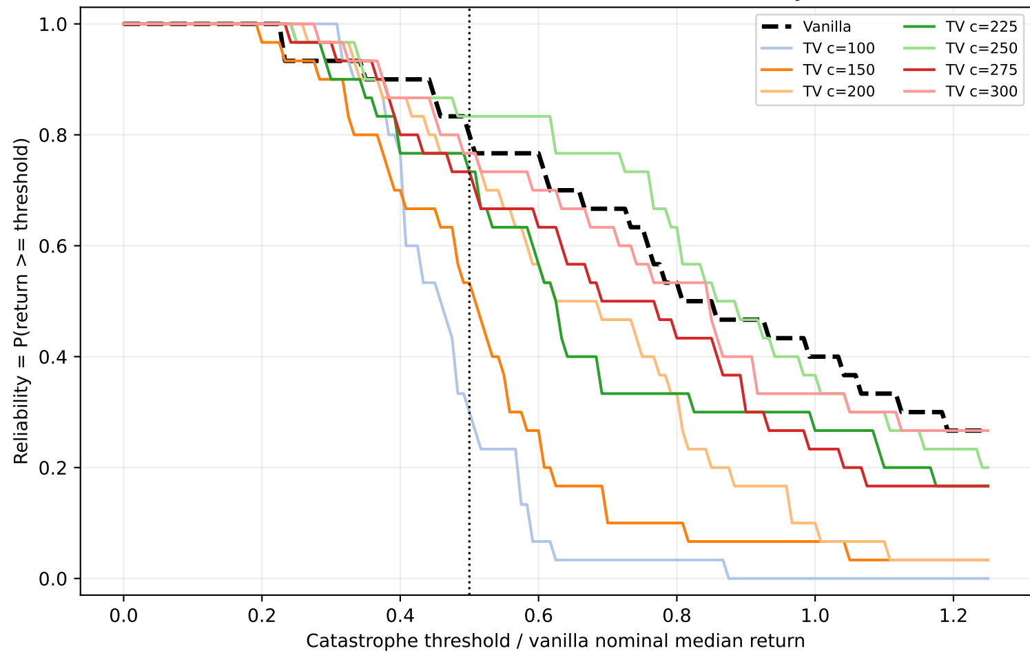
Walker2d-v4 mass factor=0.5: robustness reliability curve
