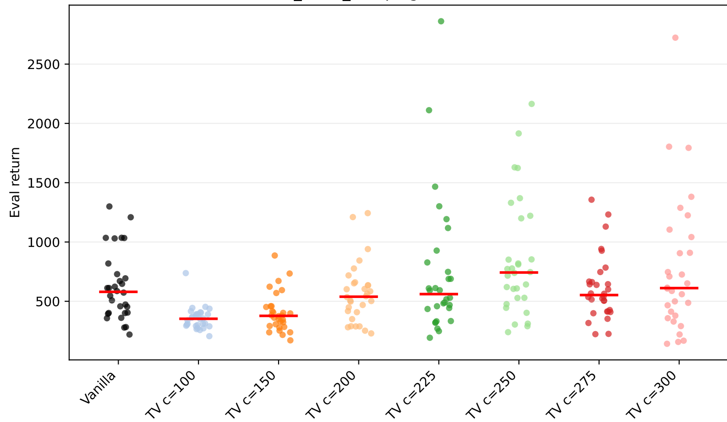
Walker2d-v4 friction_mass_damping factor=0.5: seed scatter (raw)
