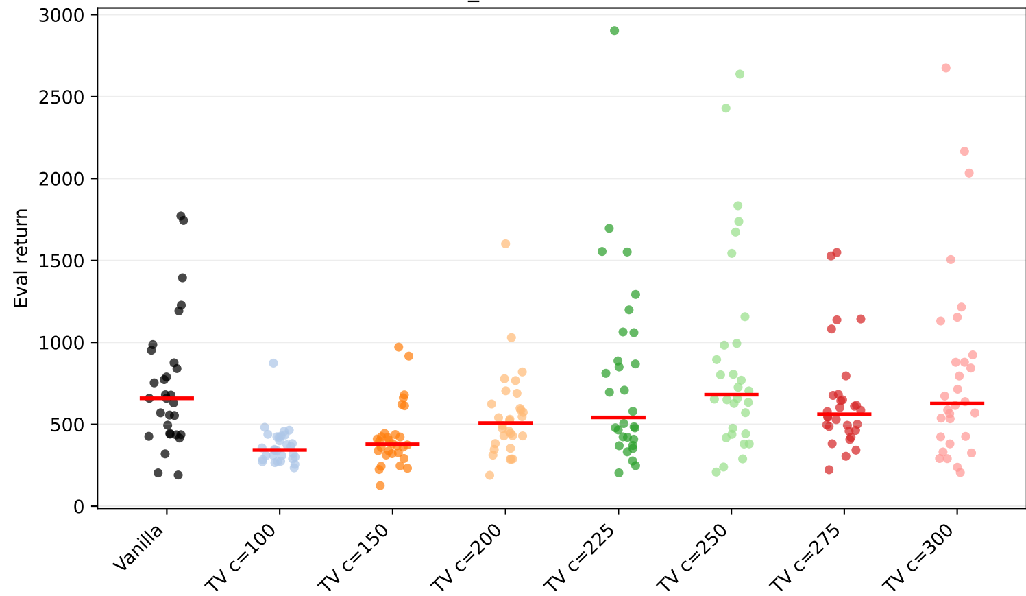
Walker2d-v4 friction_mass factor=0.5: seed scatter (raw)
