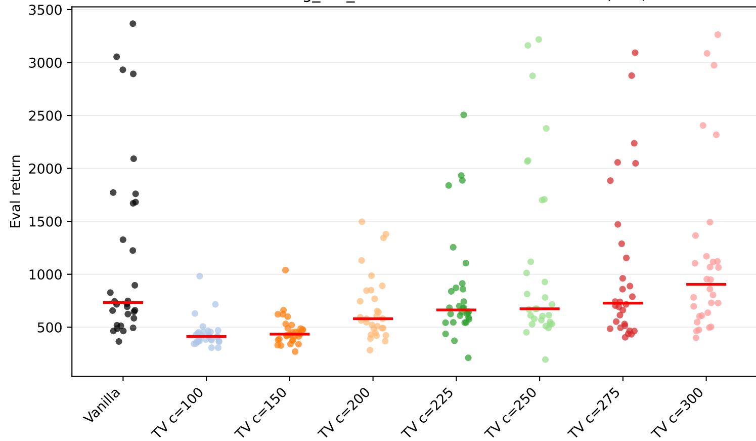
Walker2d-v4 leg_left_mass factor=0.5: seed scatter (raw)
