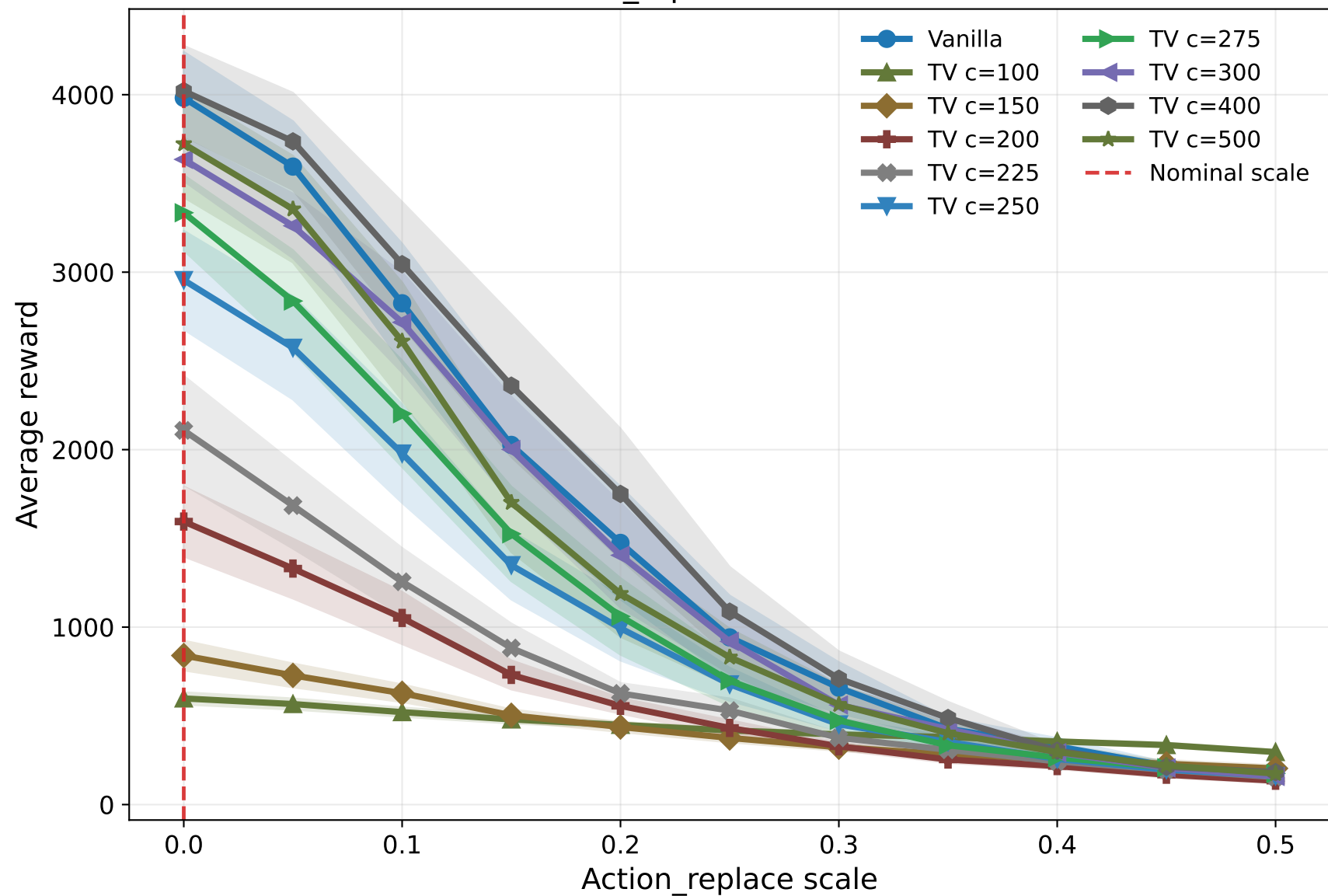
Action_replace robustness
