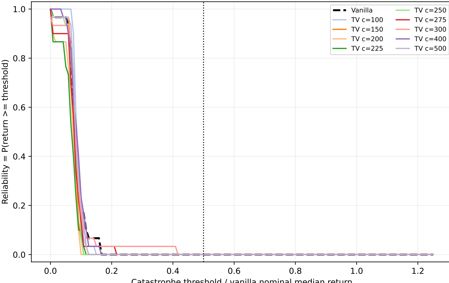
Walker2d-v5 actuator gain factor=0.5: robustness reliability curve
