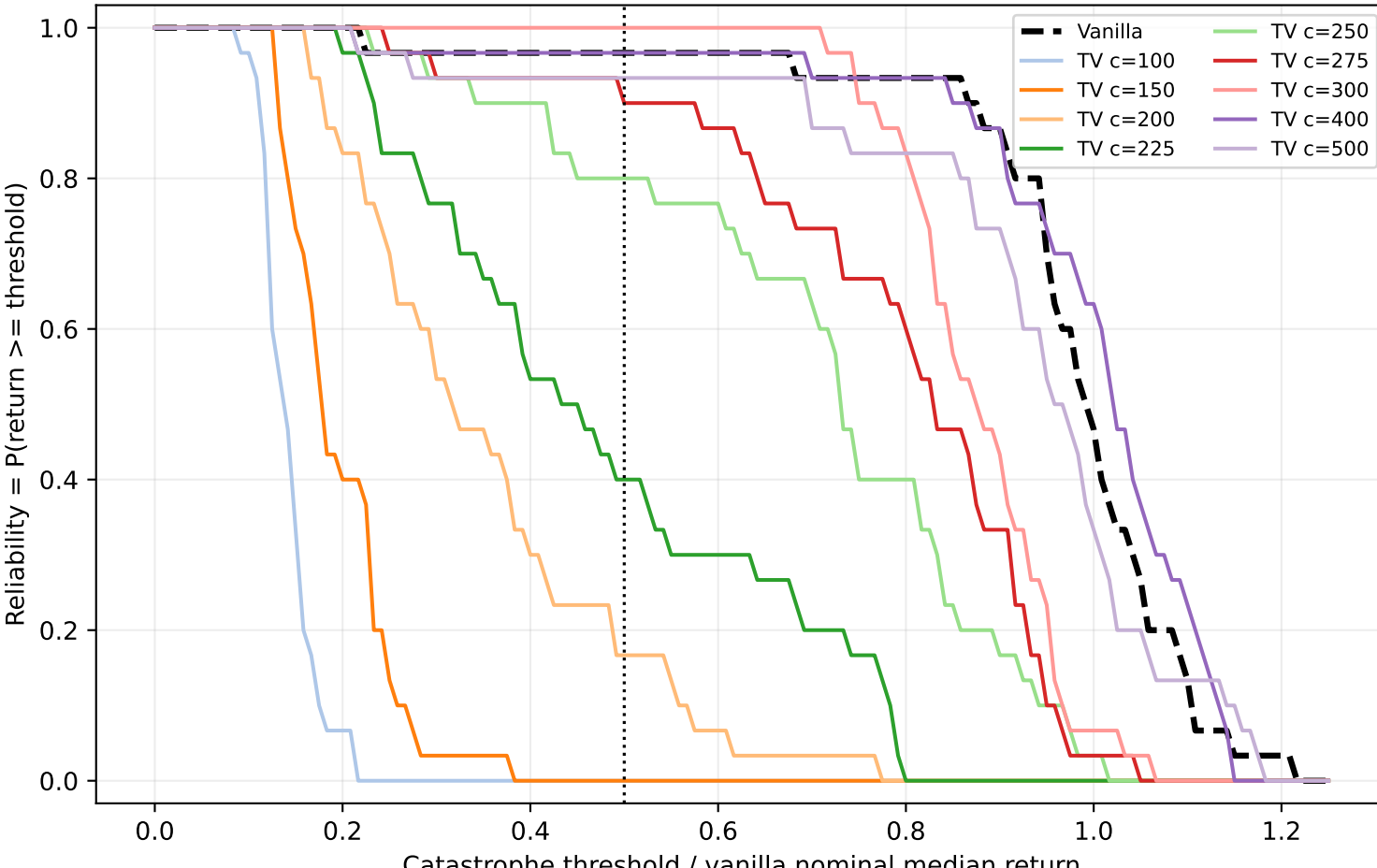
Walker2d-v5 damping factor=0.5: robustness reliability curve
