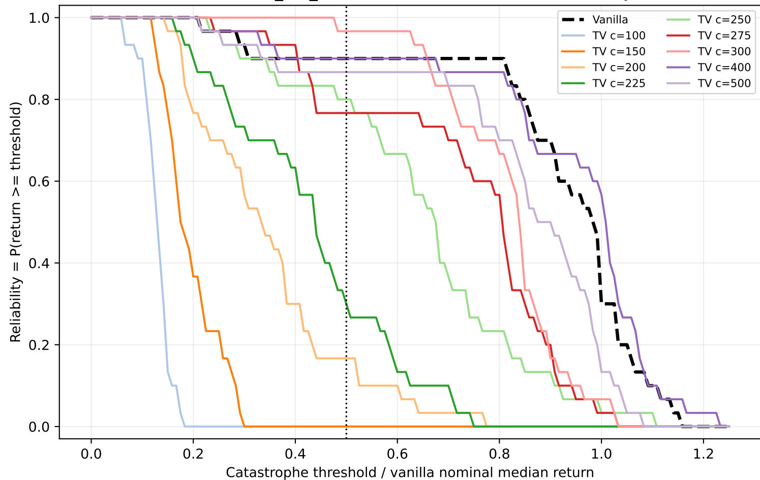
Walker2d-v5 foot_left_mass factor=0.5: robustness reliability curve
