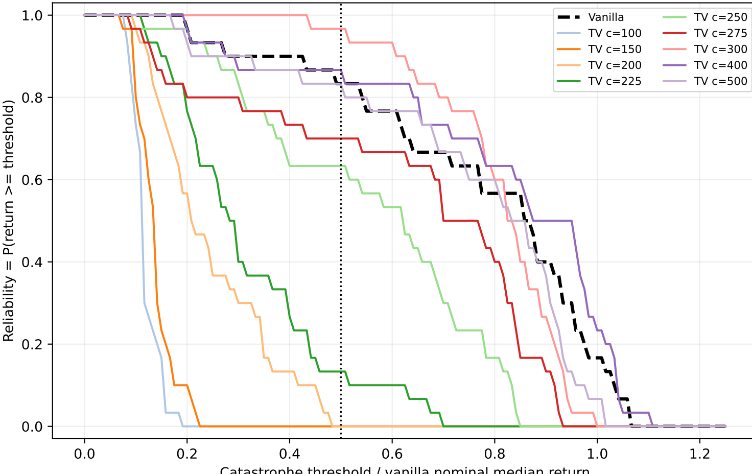
Walker2d-v5 friction factor=0.5: robustness reliability curve
