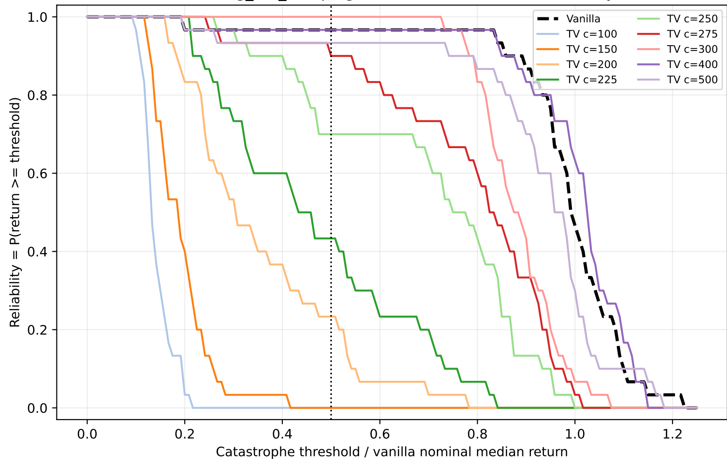
Walker2d-v5 leg_left_damping factor=0.5: robustness reliability curve
