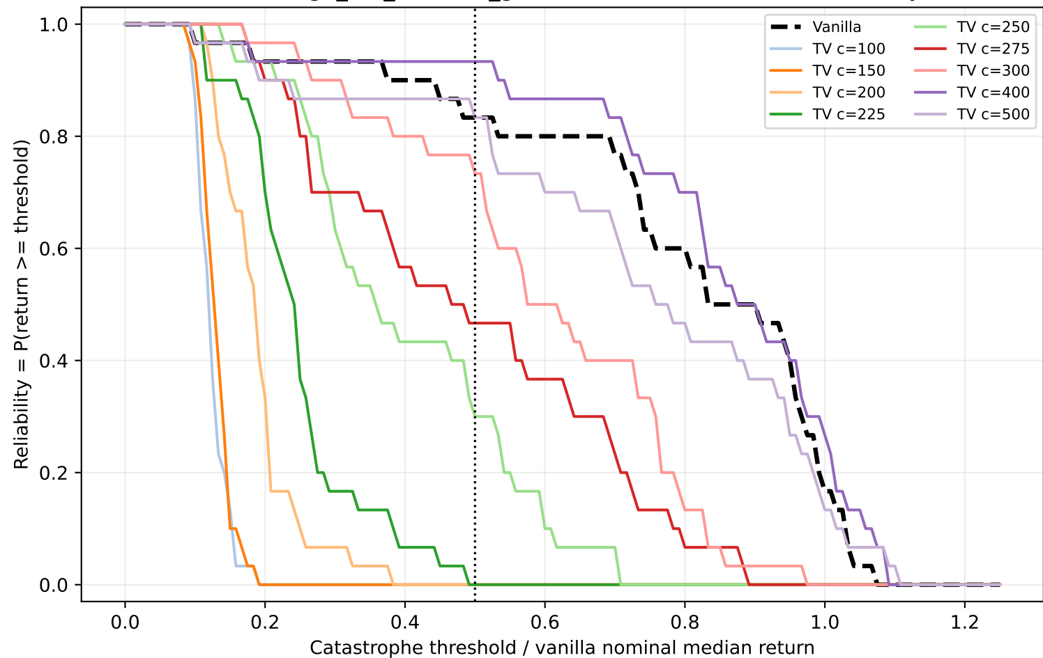
Walker2d-v5 thigh left actuator gain factor=0.5: robustness reliability curve
