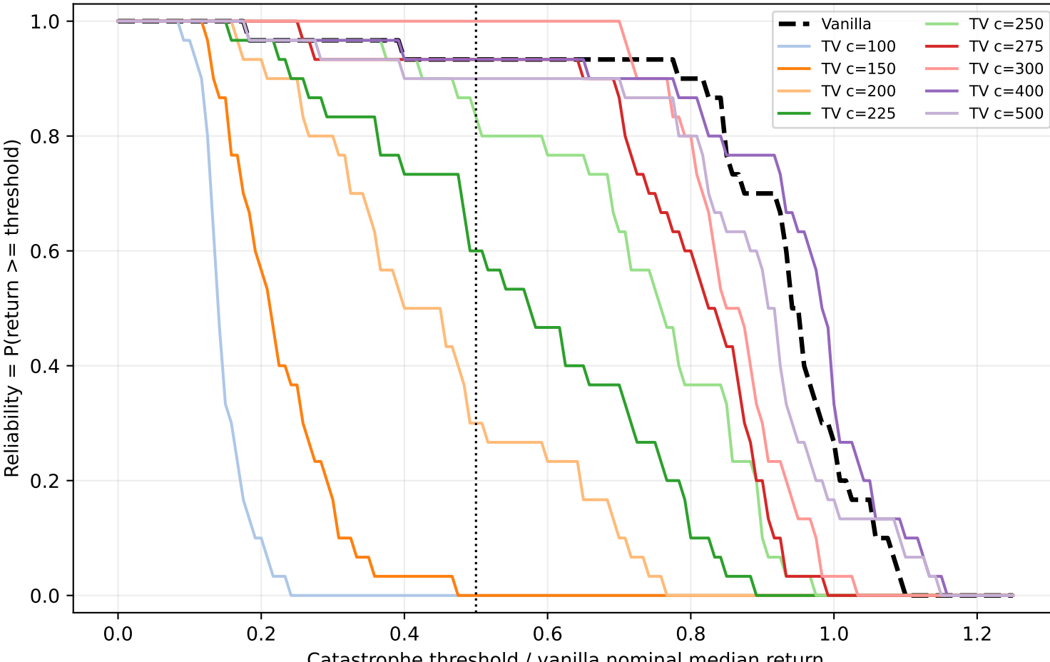
Walker2d-v5 thigh left mass factor=0.5: robustness reliability curve
