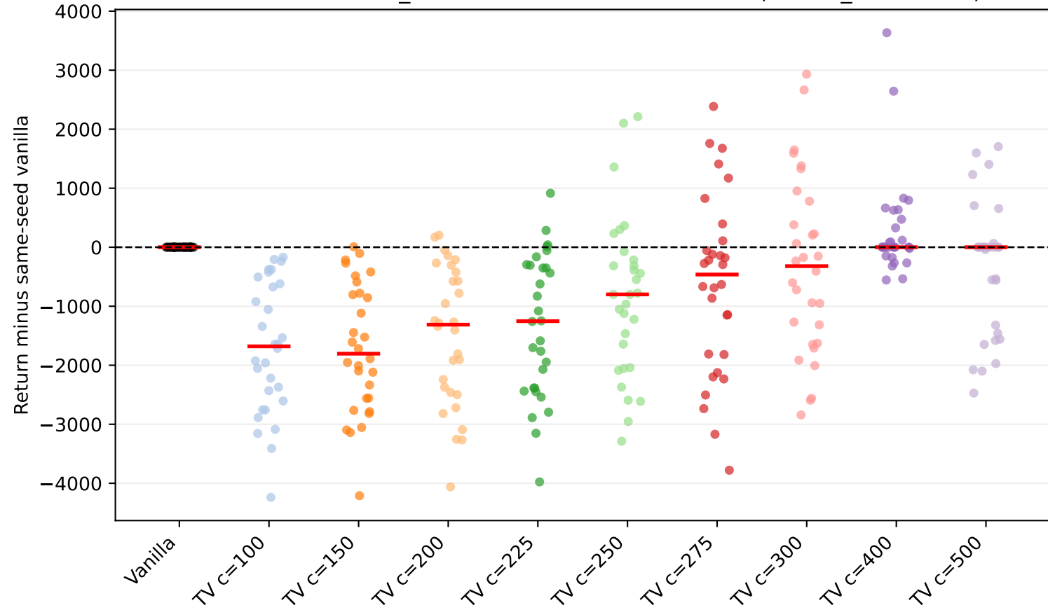
Walker2d-v5 action_noise factor=0.5: seed scatter (vanilla_subtracted)
