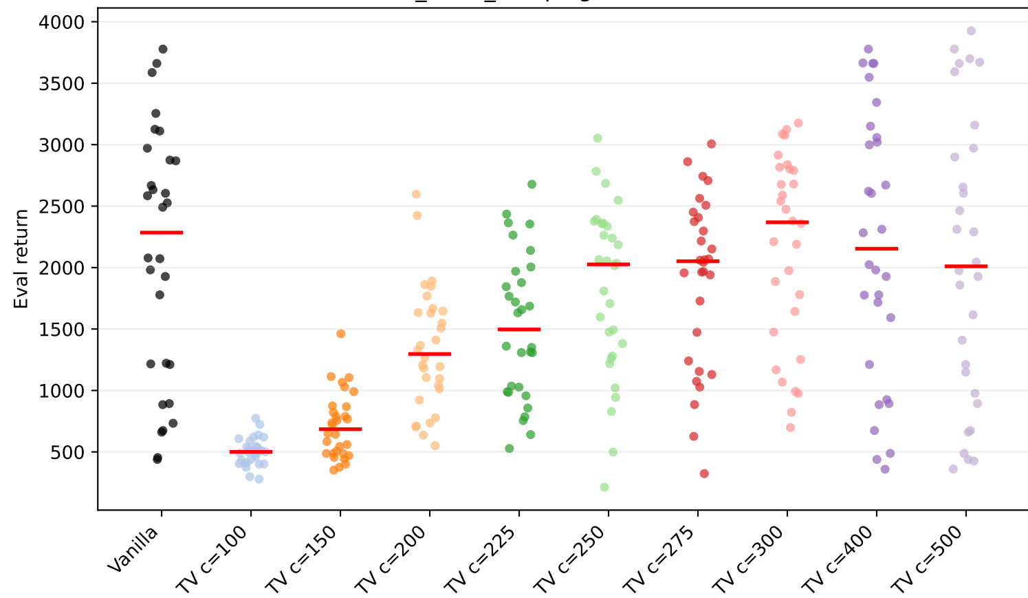
Walker2d-v5 friction_mass_damping factor=0.5: seed scatter (raw)
