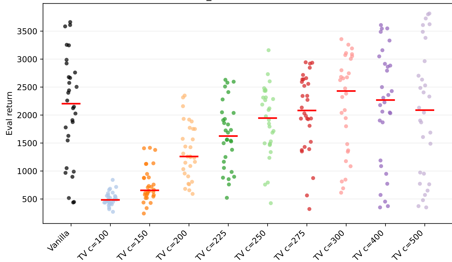
Walker2d-v5 friction_mass factor=0.5: seed scatter (raw)
