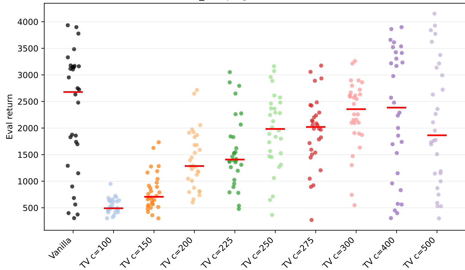
Walker2d-v5 mass_damping factor=0.5: seed scatter (raw)
